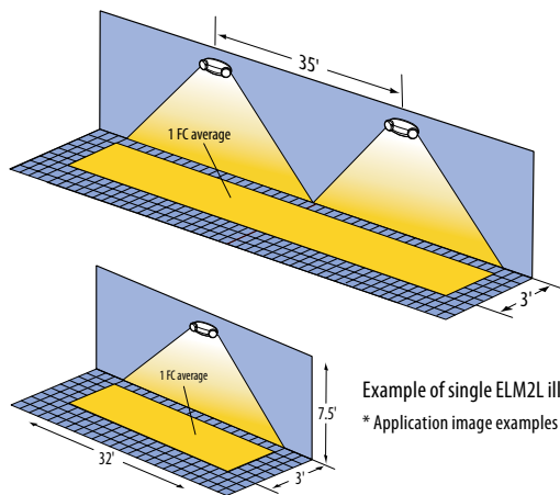
Example of multiple ELM2L luminaires illuminating a 3' path of egress.
